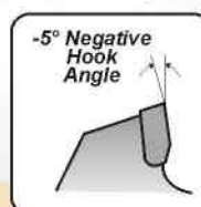
Triple Chip Grind
