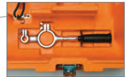
Motor handle arrangement (under the core bit)
