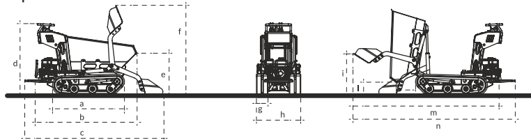
DIMENSIONS (mm)
