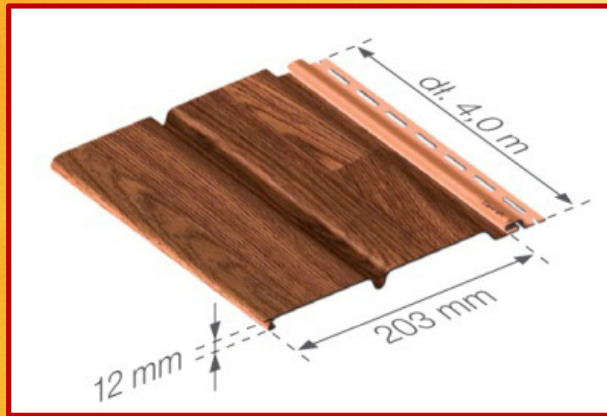
Full soffit
