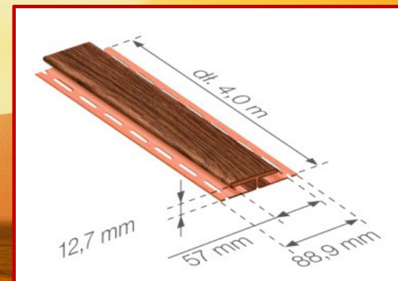
H channel
