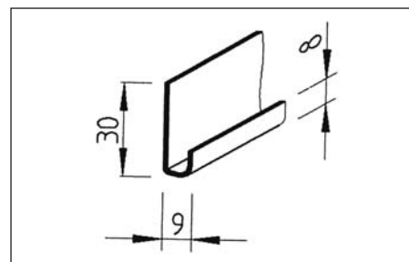
Starter Profile Standard Length 6.000 + 10 mm For Wood Cladding System
