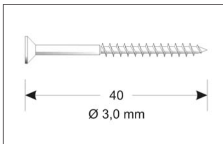
Fixing Screw 3x40 / V2A with Torx For fixing of Wood Cladding System
