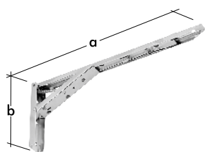
WSC - folding bracket chrome
