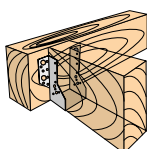
WB Joist hanger
