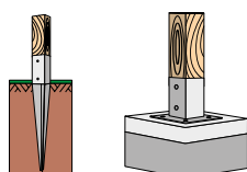
KOW / KOP Post base
