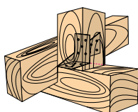
LU Plate for universal connections
