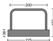
Element dublu-strat Ø 10mm
